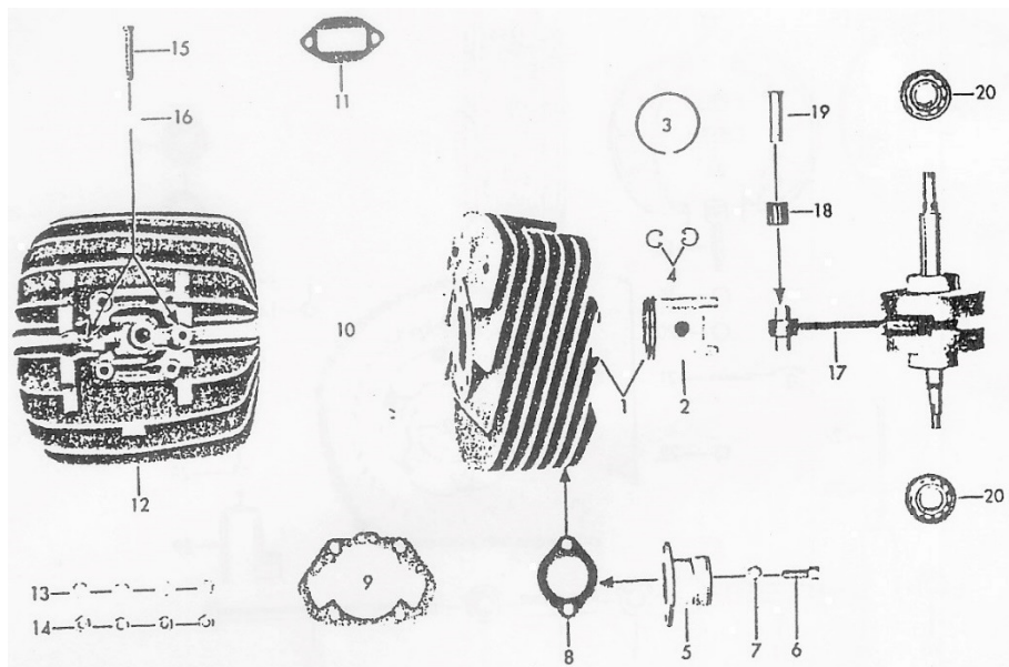
Zylinder, Kurbelwelle Cylinder, crankshaft
